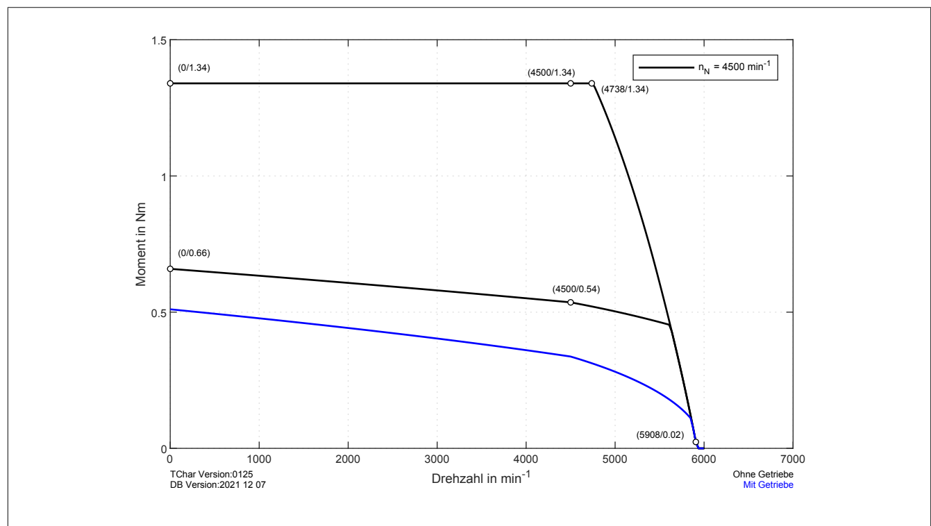
Figure 55: 8D1A22.elghijkhh-1 with 54 VDC DC bus voltage - Speed-torque characteristic curve
