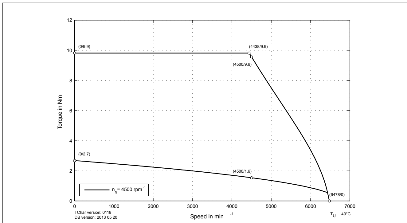
Figure 28: 8DI34e.ffggghi00-1 with 560 VDC DC bus voltage - Speed-torque characteristic curve
