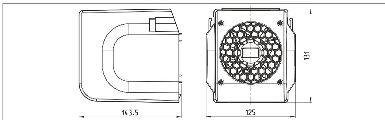
Figure 114: 8ZDFB4000000.000-0 - Dimensions
