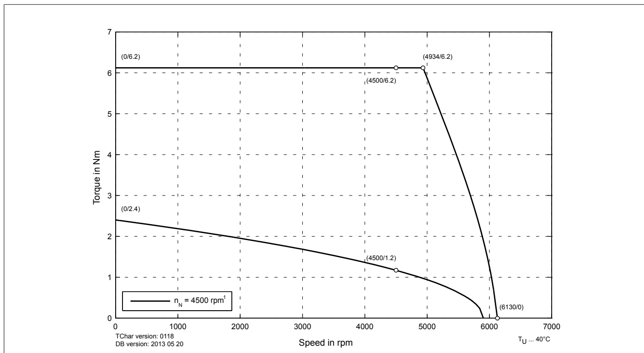
Figure 26: 8DI33e.ffggghi00-1 with 560 VDC DC bus voltage - Speed-torque characteristic curve
