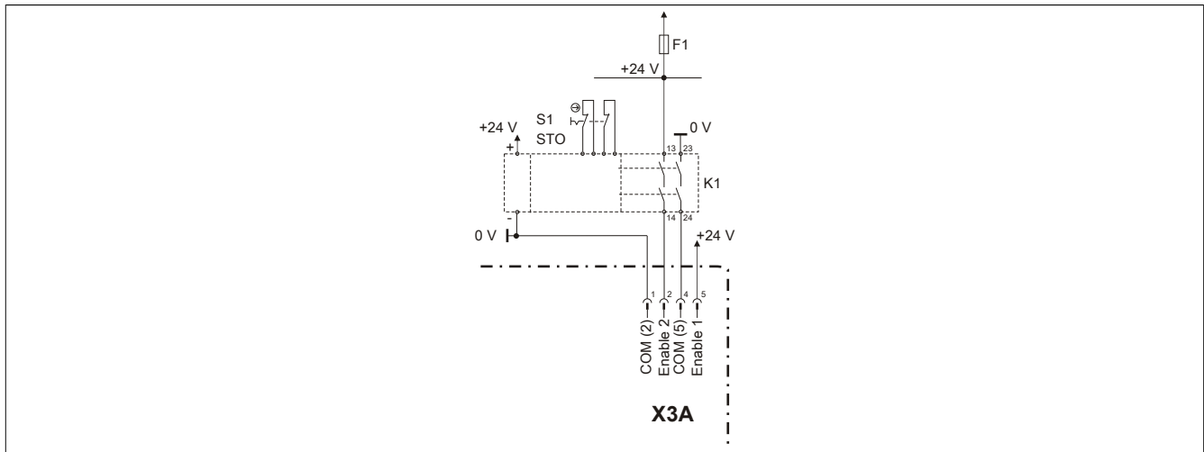
Figure 85: STO, Category 4 / SIL 3 / PL e (Variant A)
