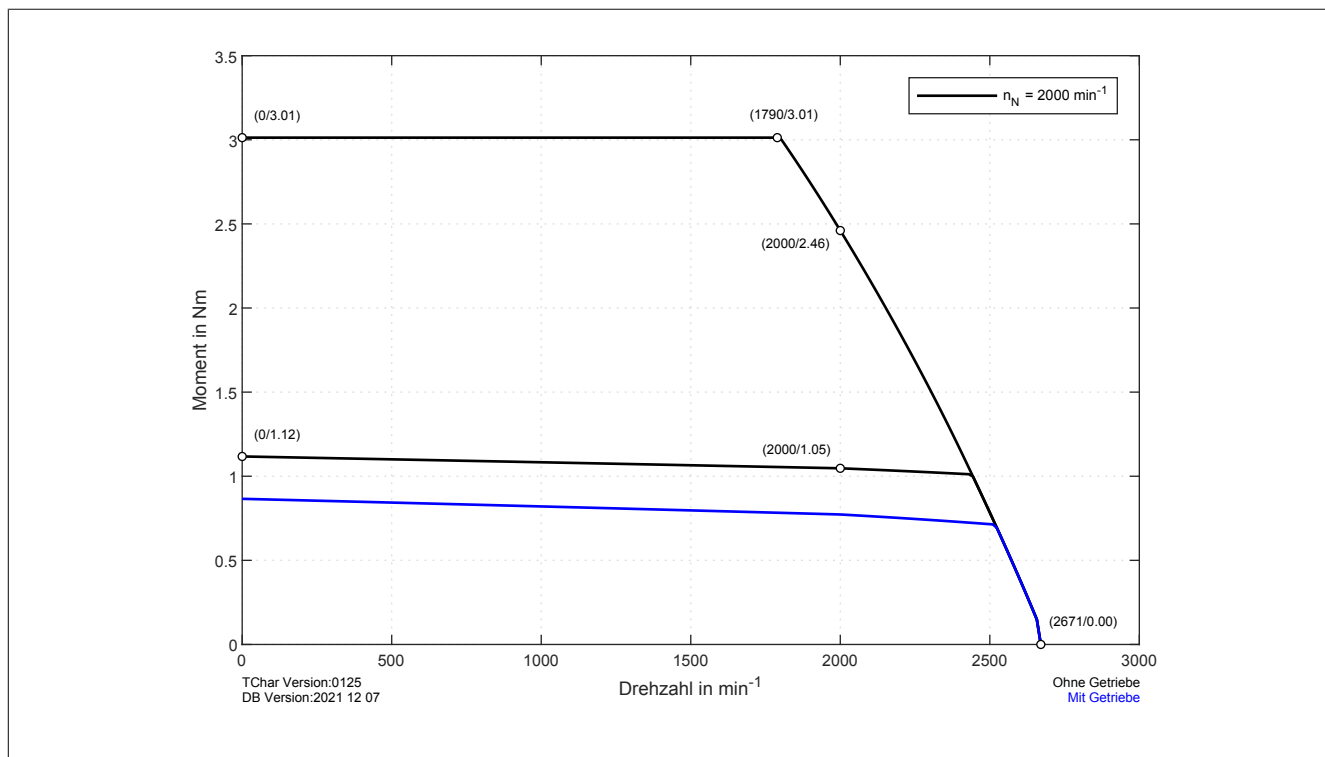
Figure 56: 8D1A23.eDghijkhh-1 with 54 VDC DC bus voltage - Speed-torque characteristic curve
