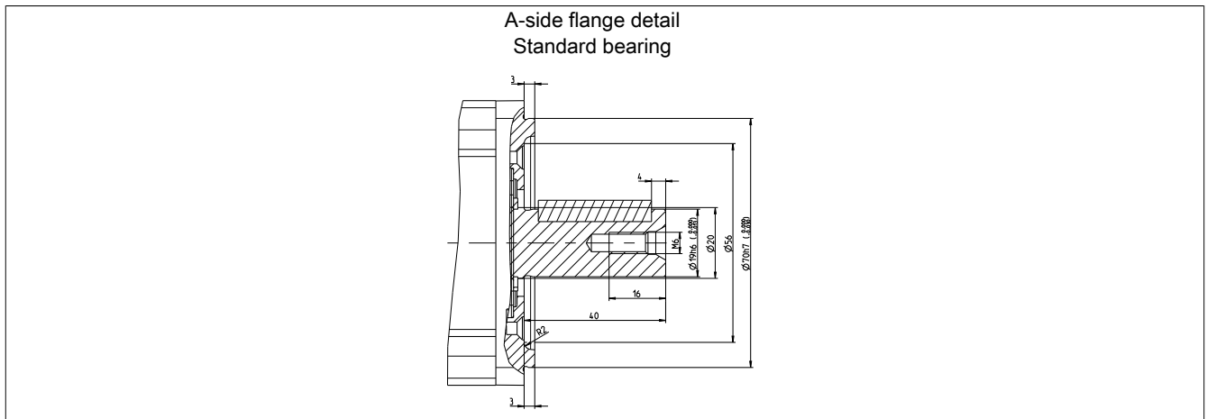
Figure 44: Flange details
