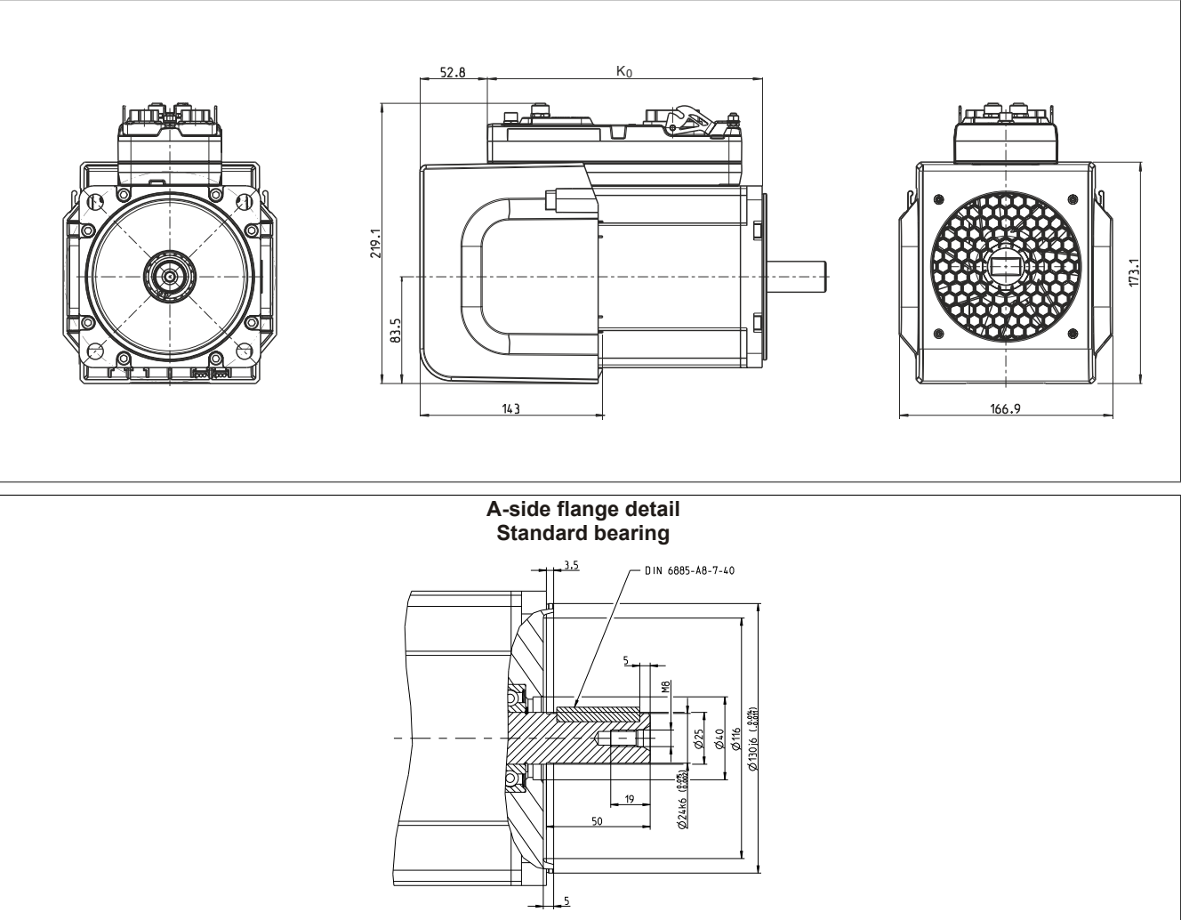
Figure 52: Flange details
