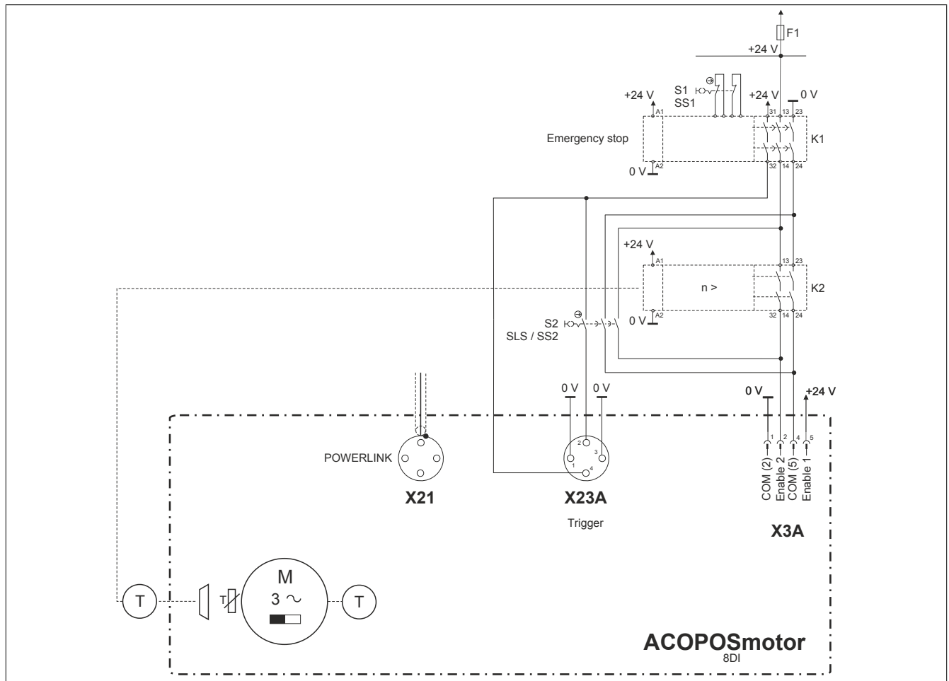
Figure 91: SS1, SLS, SS2 - Safety Category 4 / SIL 3 / PL e (Variant A)
