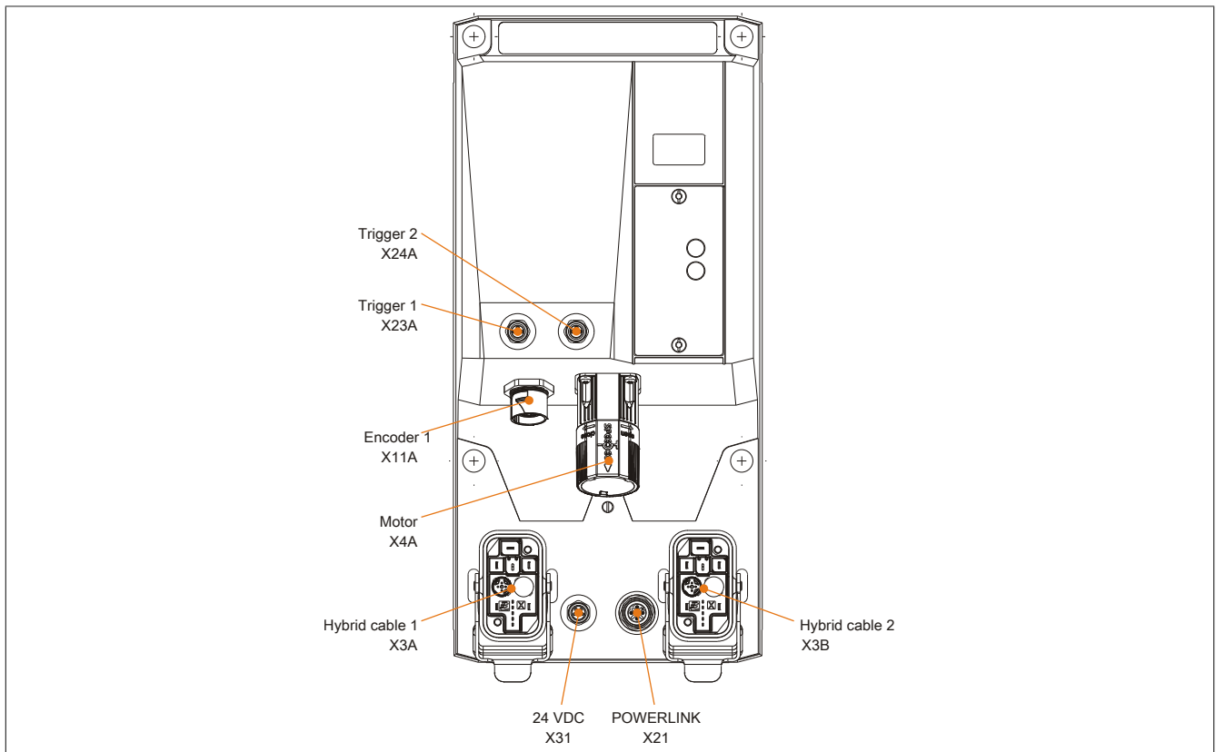
Figure 13: Pinout overview
