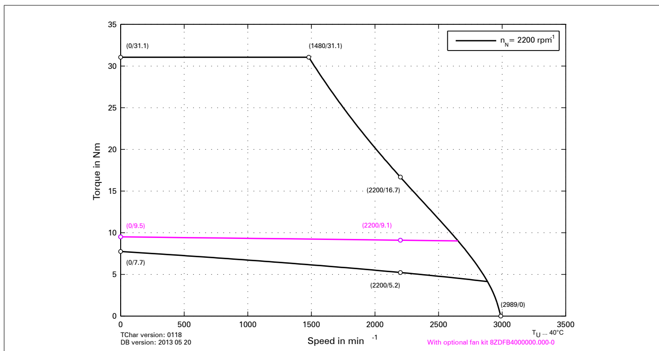
Figure 32: 8DI46e.ffggghi00-1 - Speed-torque characteristic curve
