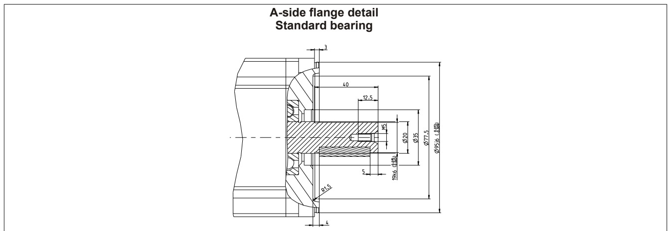
Figure 48: Flange details
