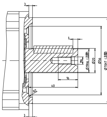
Figure 45: Flange details
