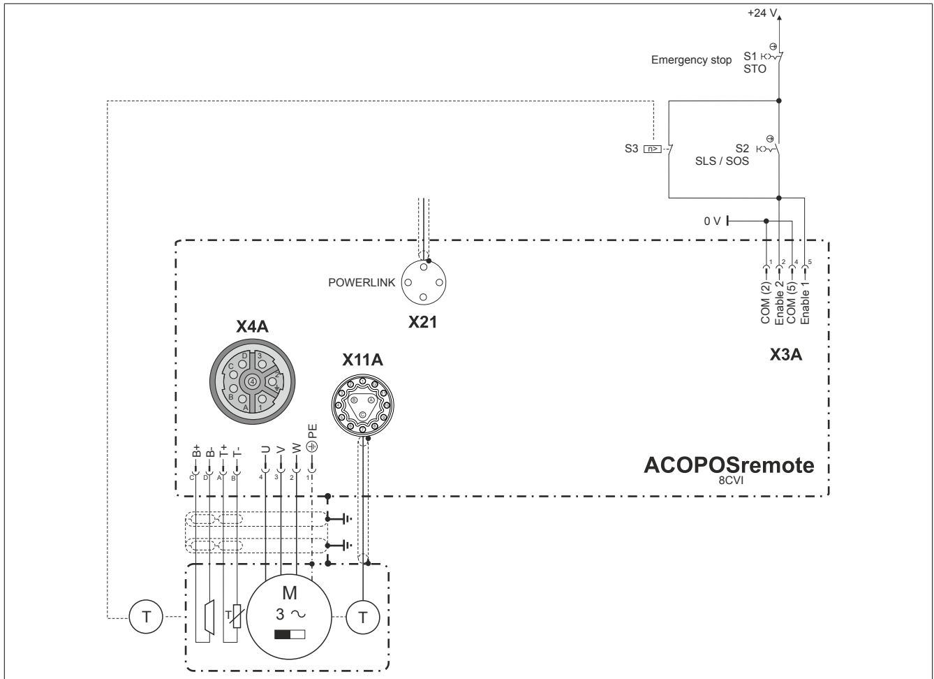
Figure 94: STO, SLS, SOS - Safety Category 3 / SIL 2 / PL d
