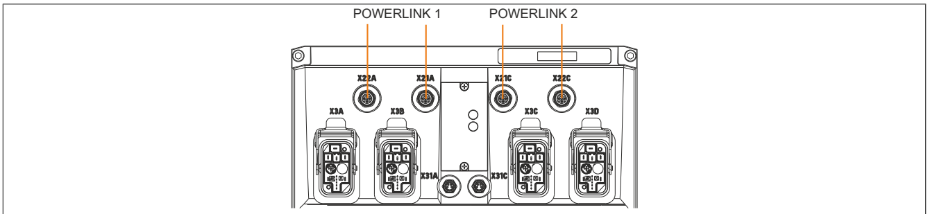
Figure 21: Cabling for 2 independent POWERLINK networks
