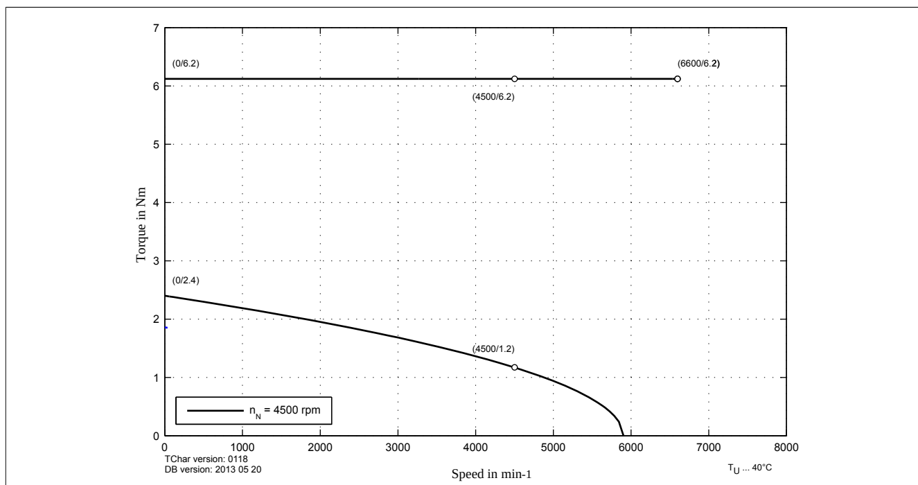
Figure 27: 8DI33e.ffggghi00-1 with 750 VDC DC bus voltage - Speed-torque characteristic curve
