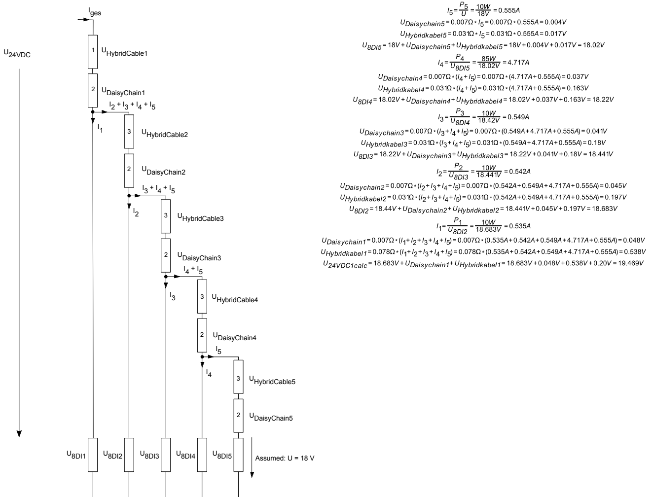
Figure 73: ACOPOSmotor drive system - Equivalent circuit diagram
