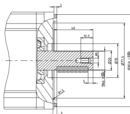
Figure 49: Flange details
