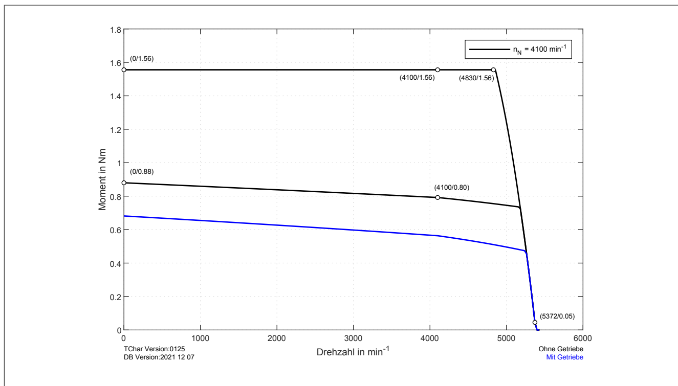
Figure 57: 8D1A23.eHghijkhh-1 with 54 VDC DC bus voltage - Speed-torque characteristic curve
