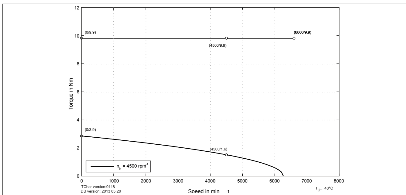
Figure 29: 8DI34e.ffggghi00-1 with 750 VDC DC bus voltage - Speed-torque characteristic curve
