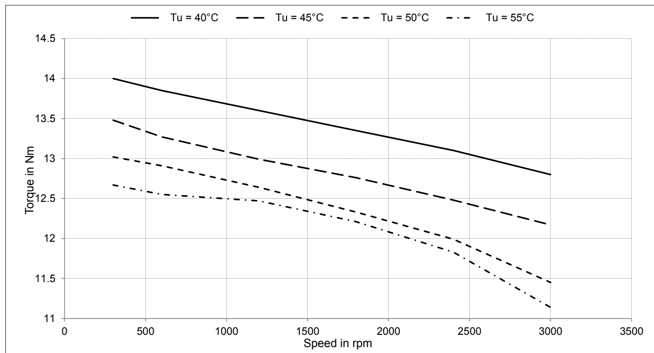
Figure 126: 8DI55e.ffggghi00-1 with optional fan kit 8ZDFB5000000.000-0
