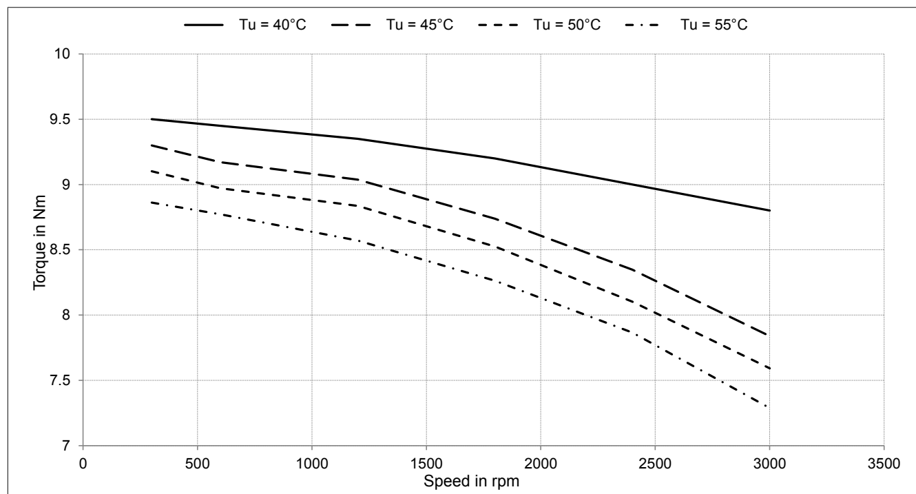
Figure 122: 8DI46e.ffggghi00-1 with optional fan kit 8ZDFB4000000.000-0
