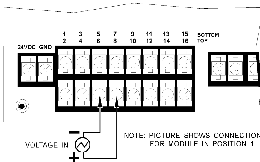
G4AD26 Connections
