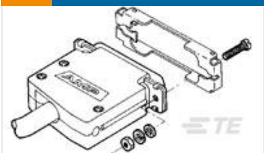
TE Part #5745584-3 UNIV SLIDELATCH KIT, SZ 3
