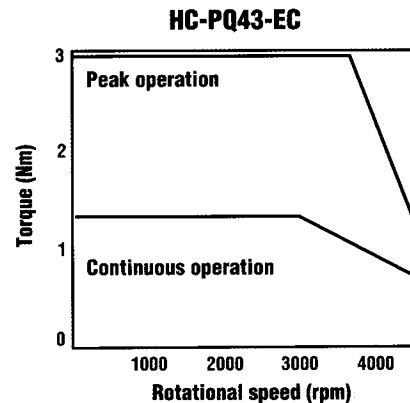
TORQUE/SPEED PROFILES
