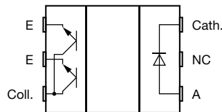
Pin connection top view
