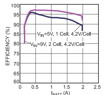
Efficiency Curve
