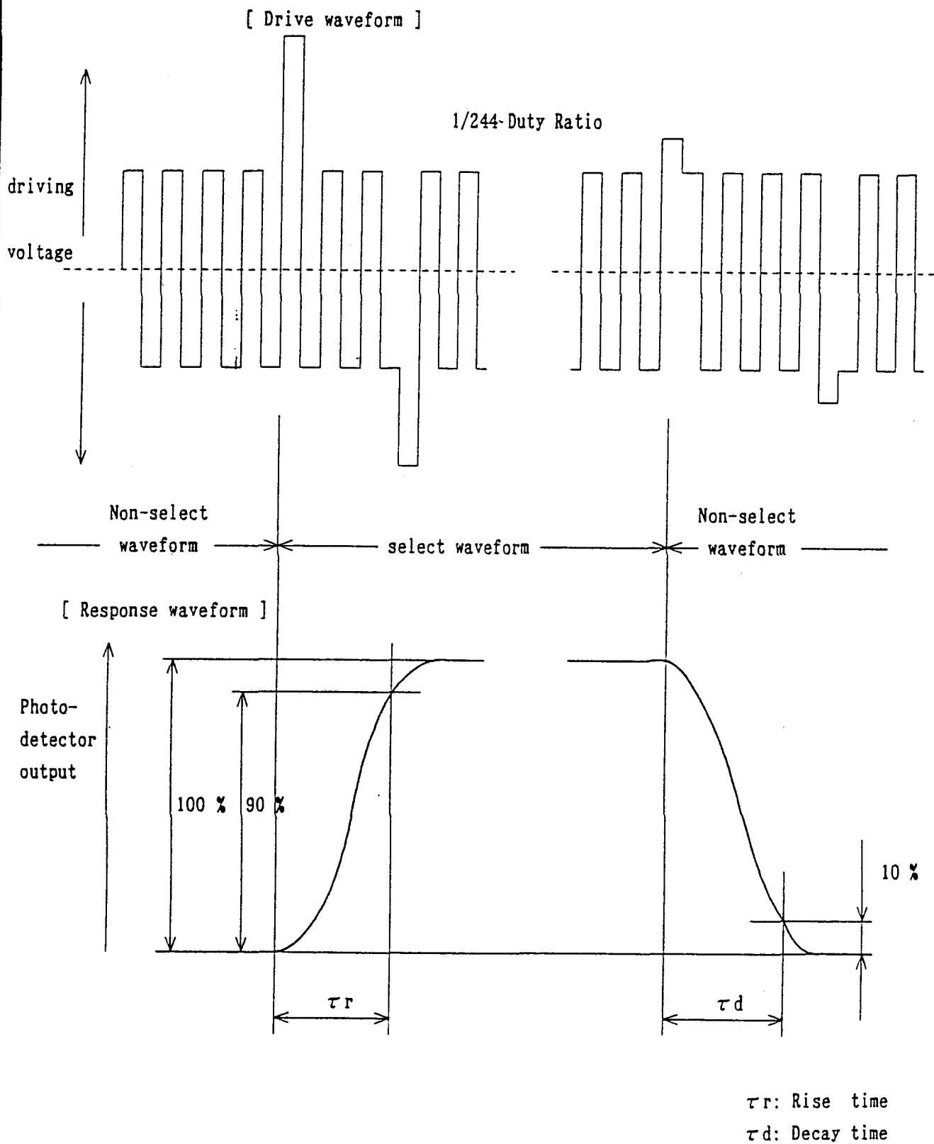
Fig.8 Definition of Response Time
