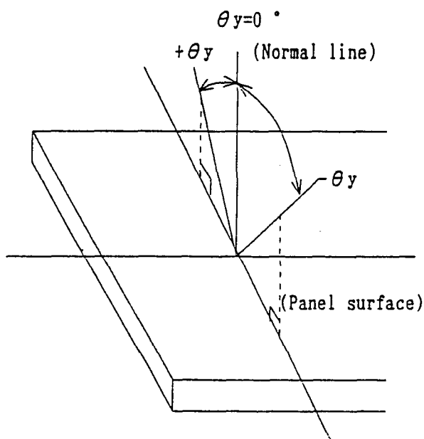
Fig.12 Dot matrix LCD viewing angle
