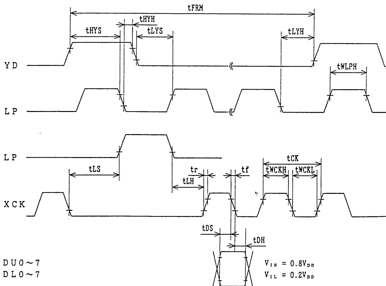
Fig.3 Interface timing chart
