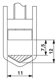
Dimensioned drawing
