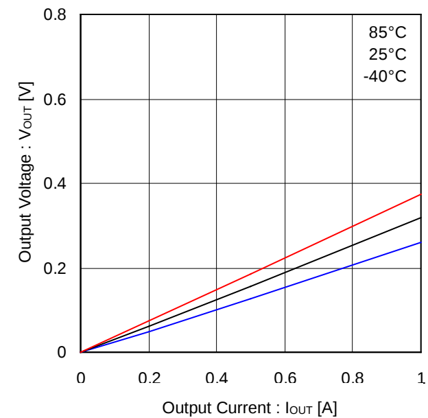
Figure 25. Output Low Voltage vs Output Current (BD6211)
