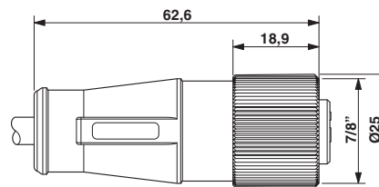
Dimensioned drawing
