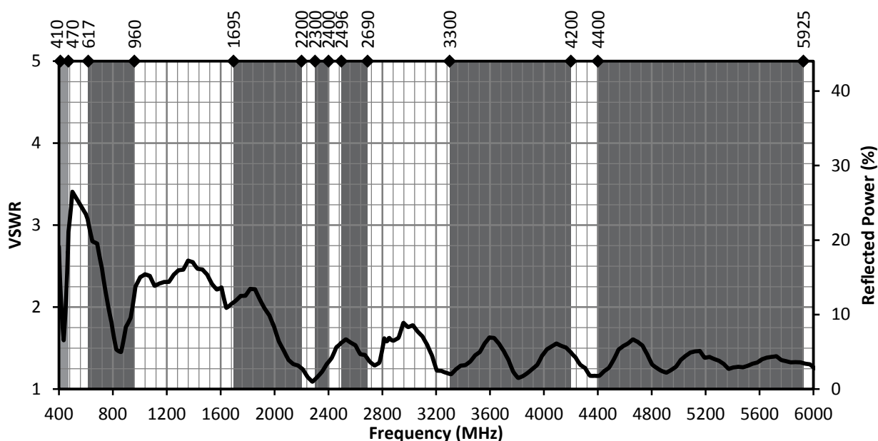
Figure 2. L001266-01 VSWR
