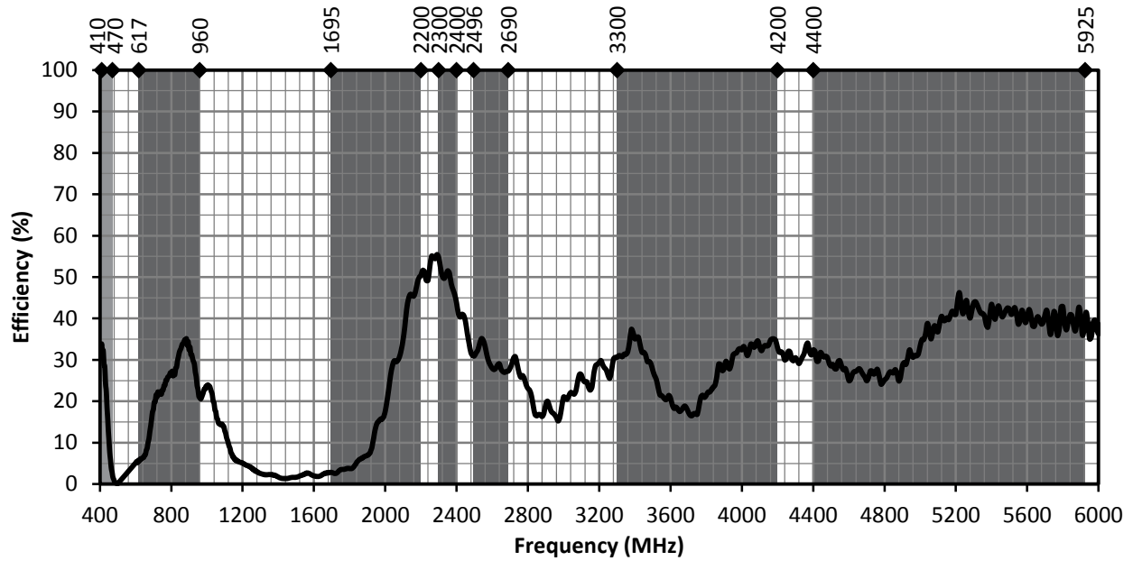
Figure 6. L001266-01 Antenna Efficiency
