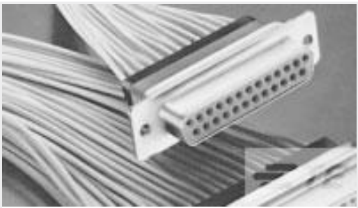
TE Part # 2-449862-3 AMPLIMITE RCPT, KIT, NM, 90, 3
