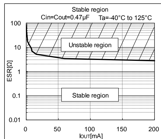
Figure 50. Stability area characteristics ( V_{IN}=1.7^{(Note1)} to 6.0V)
