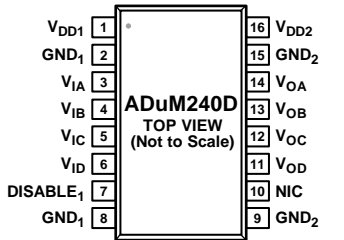
Figure 5. ADuM240D Pin Configuration
