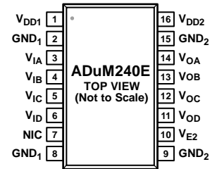
Figure 6. ADuM240E Pin Configuration
