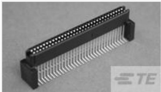
TE Part #120524-1 1FHR,64,30A/P,S,N,S14,15
