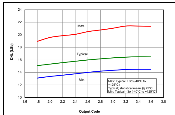
FIGURE 38-72: DAC INL Error, V_{DD} = 3.0V , PIC16LF15325/45 Only.
