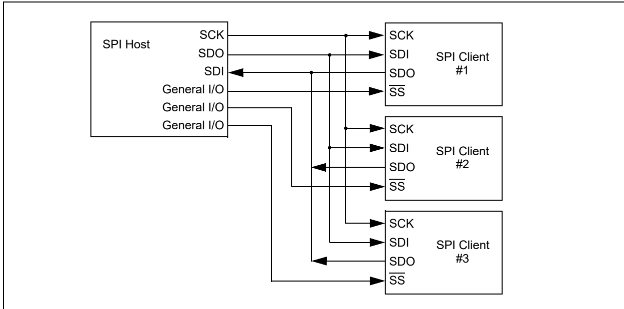
FIGURE 32-4: SPI HOST AND MULTIPLE CLIENT CONNECTION
