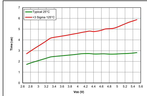
FIGURE 38-47: BOR Response Time, PIC16F15324/44 Only.
