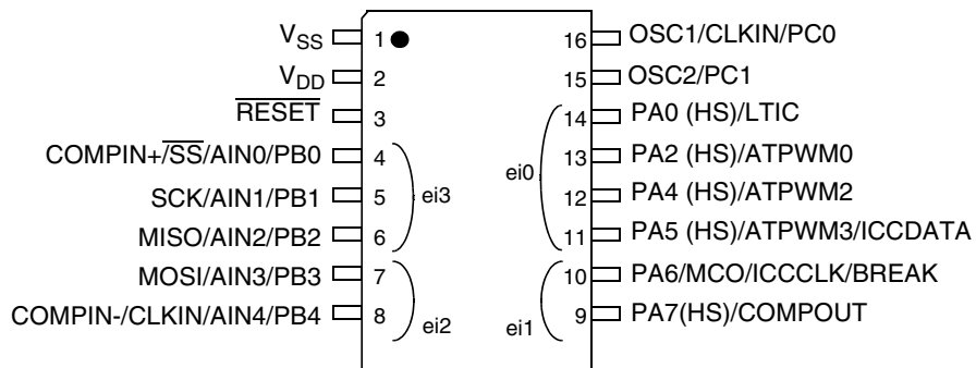
Figure 4. 16-Pin SO and DIP Package Pinout
