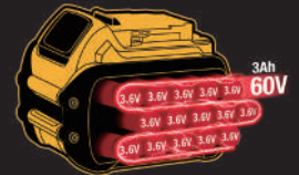
Series connection
