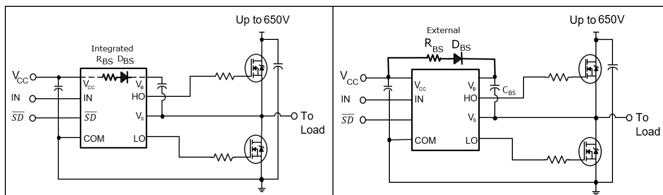
Figure 15 2ED218x with integrated components
