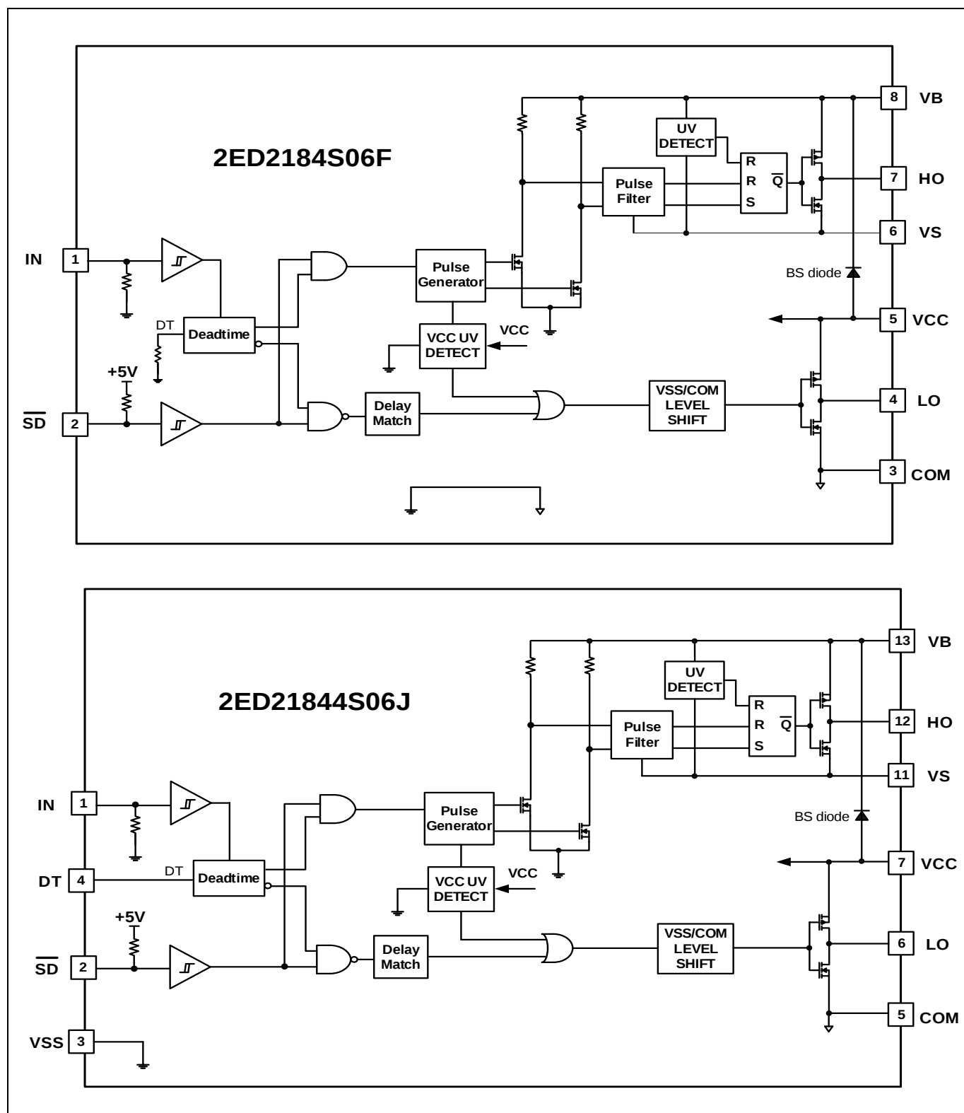
Figure 2 Block diagrams
