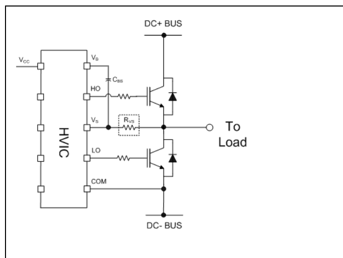
Figure 26 Resistor between the V_S pin and the switch node
