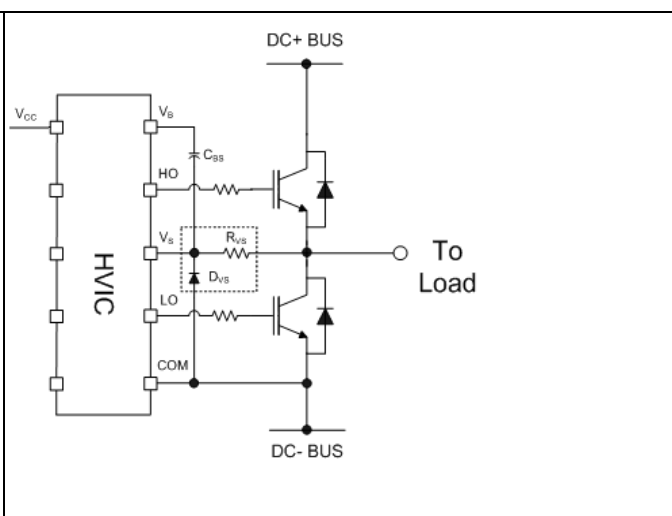
Figure 27 Clamping diode between COM and V_S
