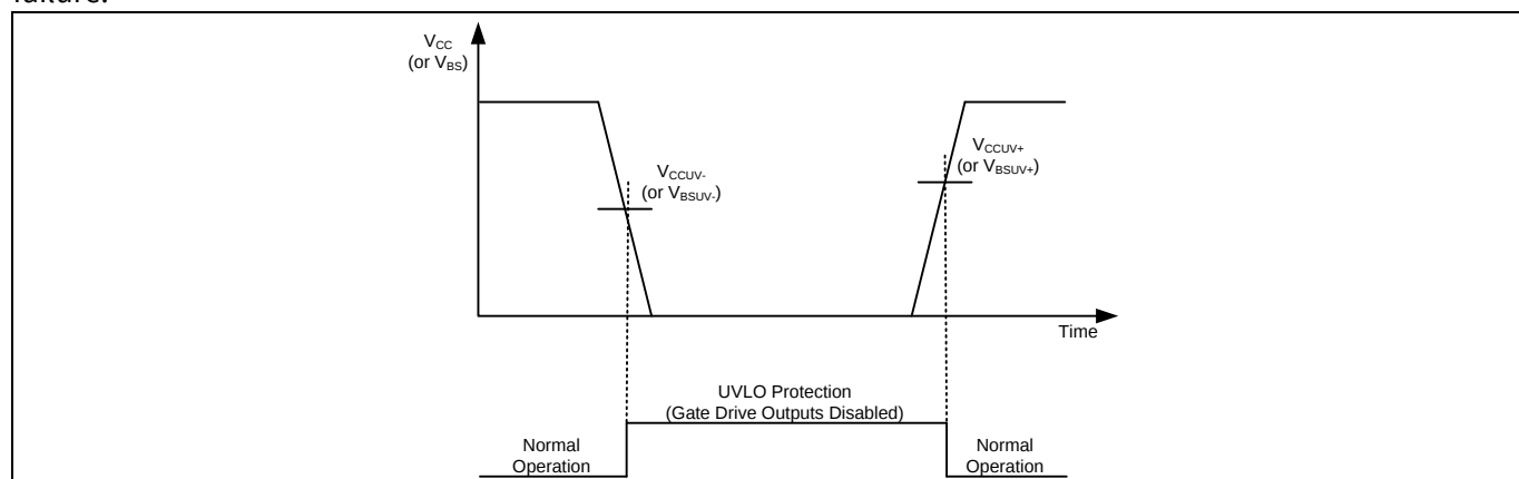
Figure 13 UVLO protection
