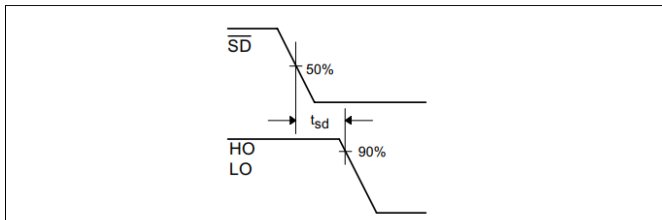
Figure 14 Shutdown waveform definitions
