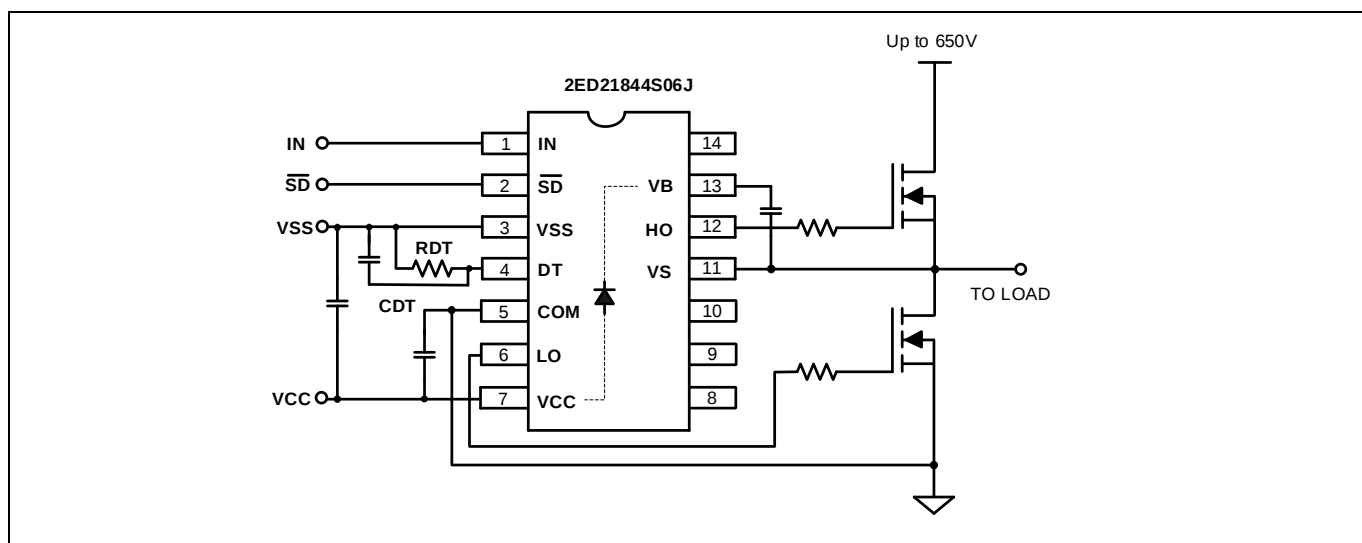
Figure 10 14-pin half-bridge variants having adjustable dead-time feature settable with a resistor
