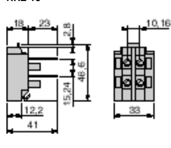
Termination adaptor RHZ-15
