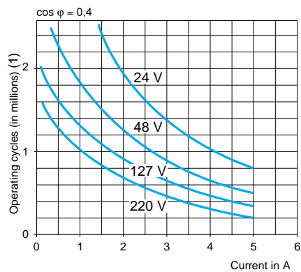
Curves at 1 operating cycle/second
