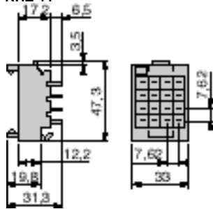
Sockets RHZ-11
