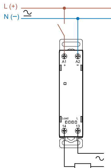
Single-phase connection (77.11/77.21)
