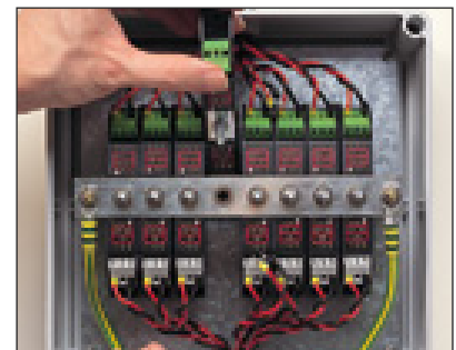
CME kits allow the simultaneous mounting and earthing of protectors through their central earth stud. Once installed, single protectors can be changed without removing others
