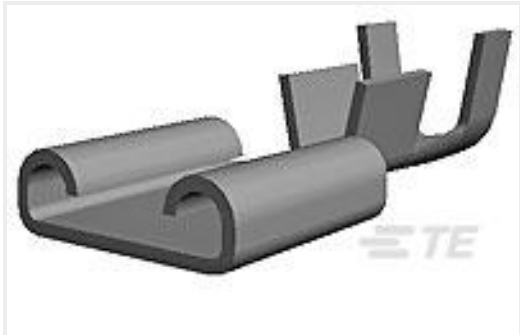
TE Part #6-160465-0 250 FASTON REC 18-16 AWG TPBR
