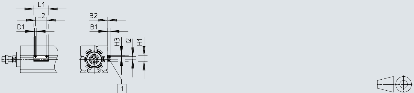
Dimensions – Sensor bracket EAPM-L2
