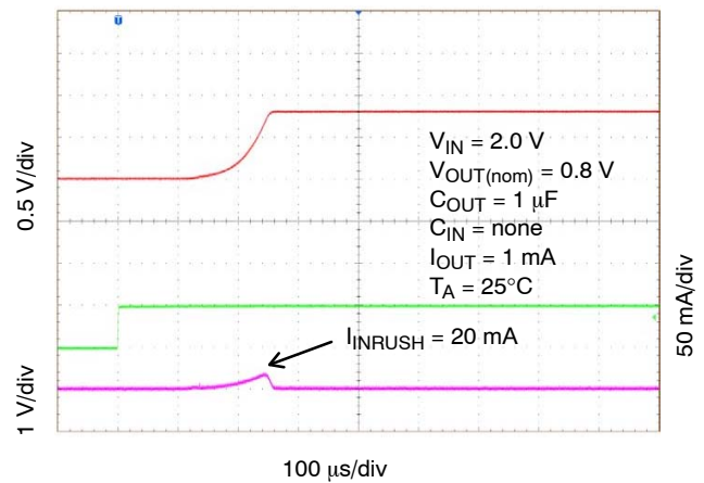
Figure 38. Enable Turn-On Response, V_{OUT} = 0.8 V , C_{OUT} = 1 \mu F
