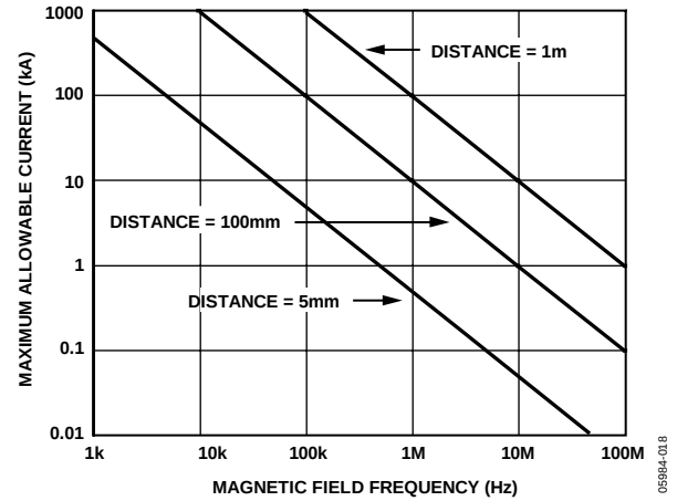
Figure 17. Maximum Allowable Current for Various Current-to-ADuM330x Spacing
