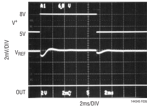
Figure 3b. V^+ Glitching Response
