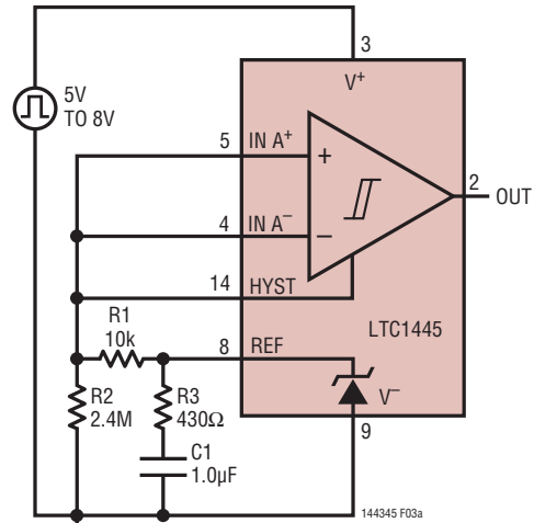
Figure 3a. V^+ Glitching Test Circuit
