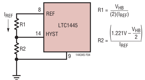
Figure 4. Programmable Hysteresis
