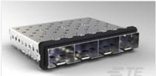
TE Part #2057833-1 SFP+ Enhanced 1x4 Cage Assy
