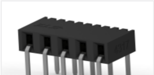
TE Part #2307706-5 5P,2MM,B-B,REC,SRHZ,2.1,0.38AU,TR
