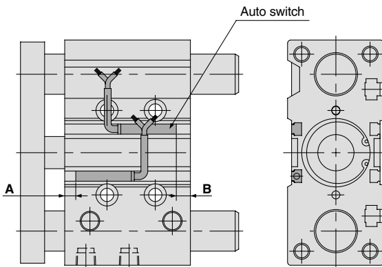
Proper mounting position (mm)
