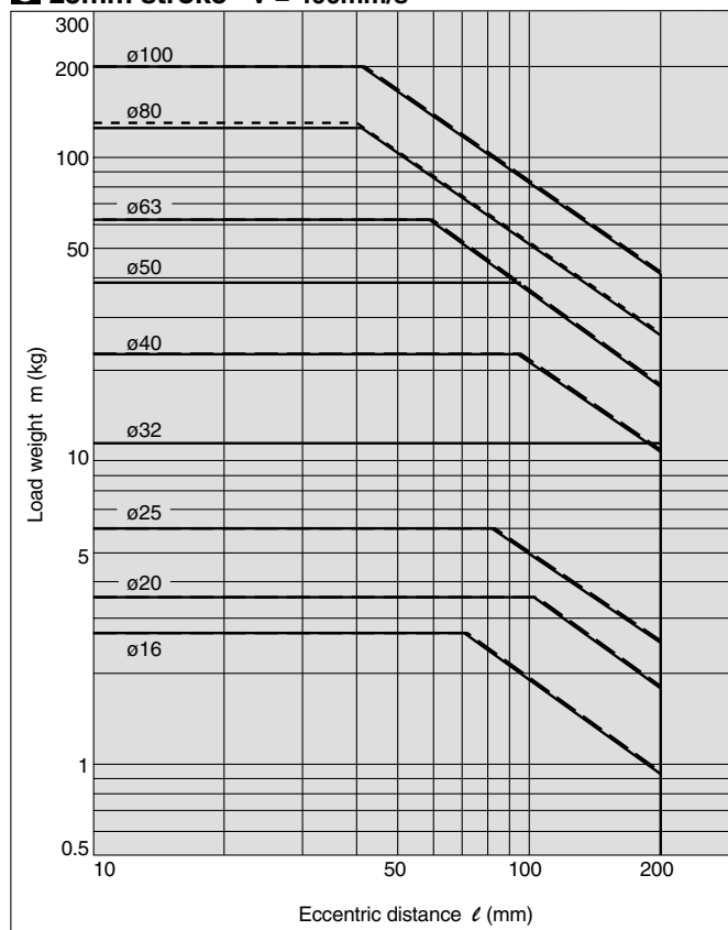
3 25mm stroke V = 400\text{mm/s}
