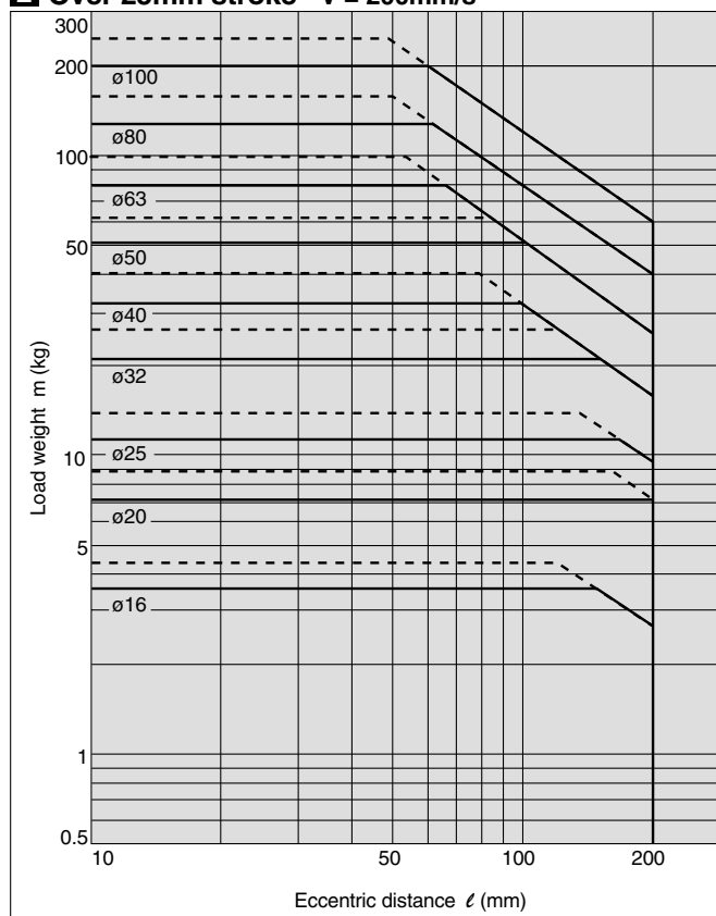
2 Over 25mm stroke V = 200\text{mm/s}
