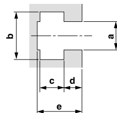
T-slot dimensions
