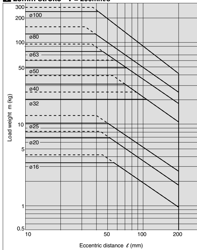
1 25mm stroke V = 200\text{mm/s}
