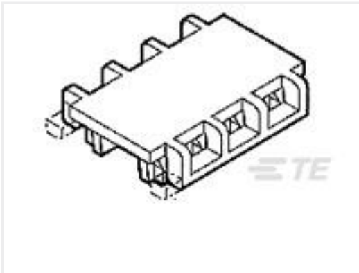
TE Part #1-643071-2 12P MTA156 FD-THRU COVER
