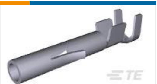
TE Part #350536-6 UMNL SOK 20-14 .0125AUNI/PHBZ
