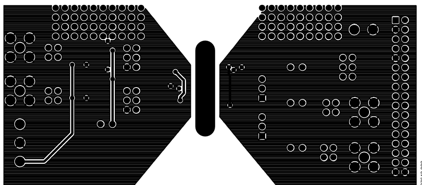
Figure 8. Solder Side Artwork for the EVAL-AD7401A, 16-Lead SOIC Package
