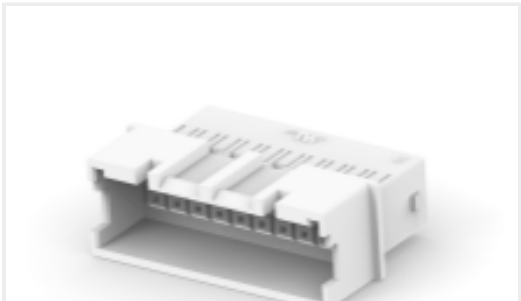
TE Part # 2-2324201-0 HSG,REC,FREE-HANGING,GWT, DUALROW,EP2.5
