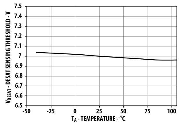
Figure 19. V_{DESAT} Threshold vs. temperature
