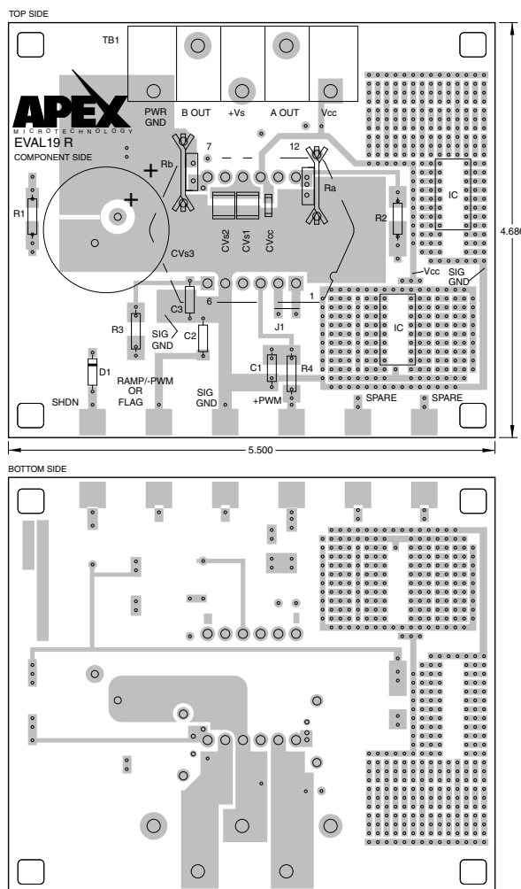
Figure 1: PCB
