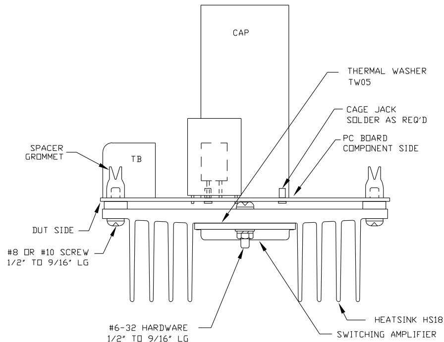
Figure 4: Mechanical Drawing
