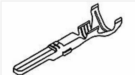
TE Part #171631-2 070 TAB CONT GOLD
