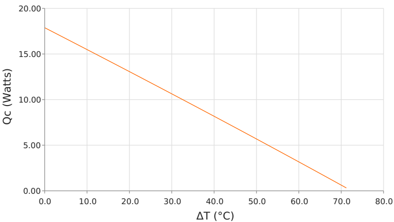
Heat Pumped at Cold Side ( Q_c ) T_{hot} = 35^\circ\text{C} | operating = 3.4 Amps
