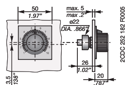
CT-POT.03 - Potentiometer 10.5 mm
