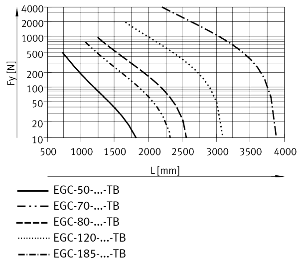
Fig. 6: The support distance L as a function of force F_y
