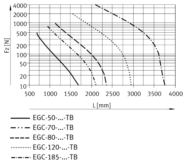
Fig. 7: The support distance L as a function of force F_z
