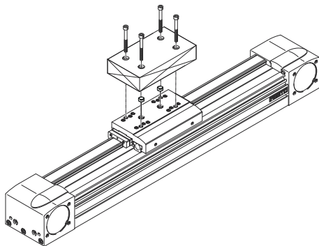
Fig. 3: Mounting payload, example "top mounting"
