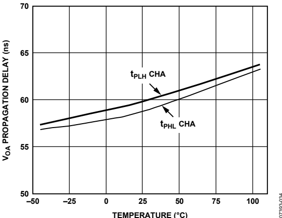
Figure 14. Typical Channel A Propagation Delay vs. Temperature
