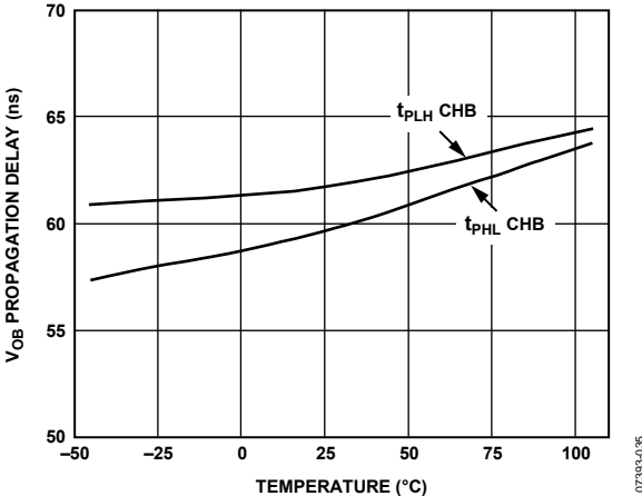
Figure 15. Typical Channel B Propagation Delay vs. Temperature
