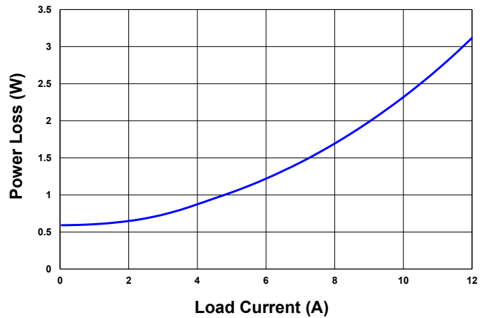
Figure 4-11. Typical Power Loss (PVIN = 12V, V OUT = 1.0V)
