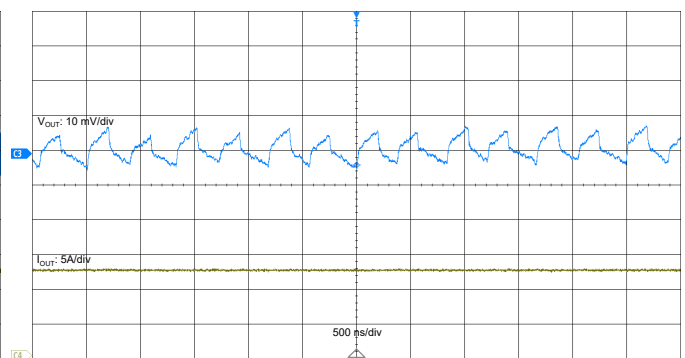
Figure 4-23. V_{OUT} Ripple
