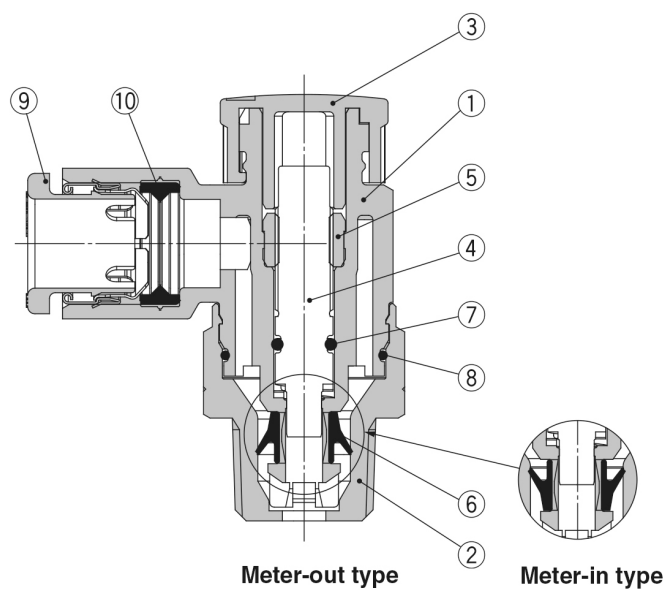
Component Parts
