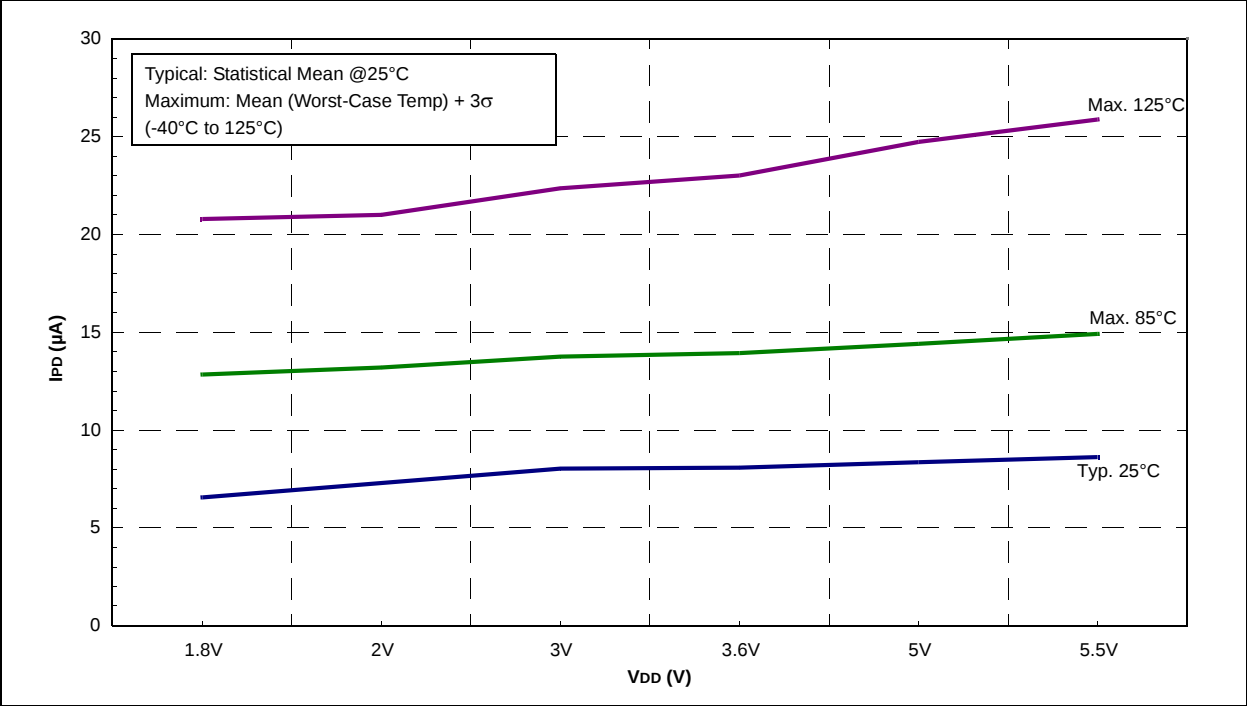
FIGURE 24-39: PIC16F72X CAP SENSE LOW POWER I_{PD} vs. V_{DD} , V_{CAP} = 0.1\mu F
