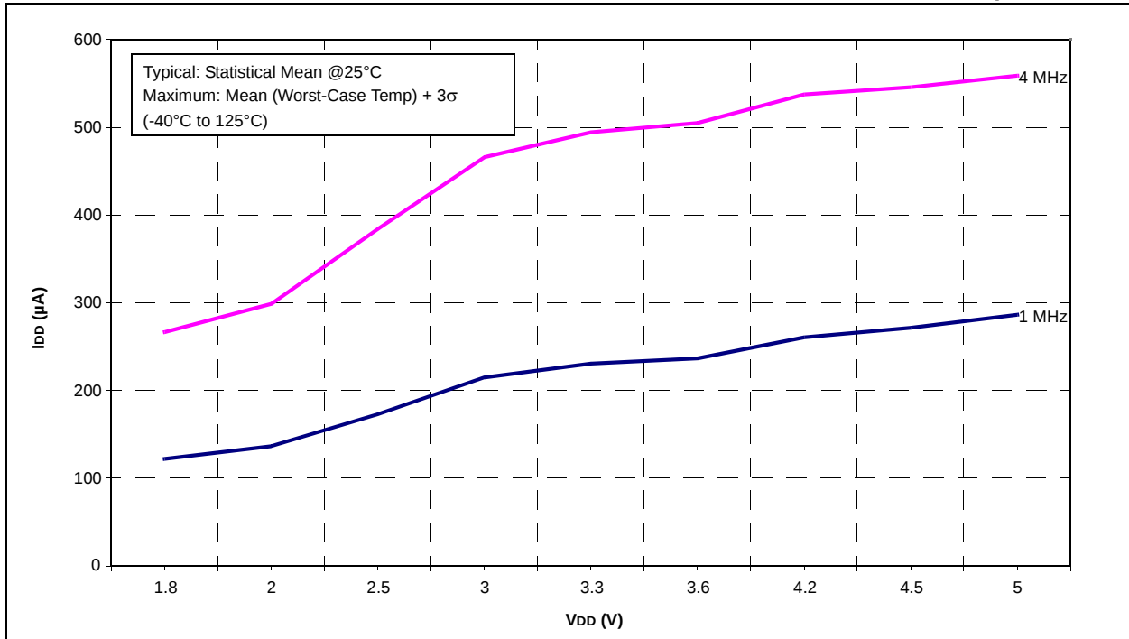
FIGURE 24-13: PIC16F72X MAXIMUM I_{DD} vs. V_{DD} OVER F_{OSC} , XT MODE, V_{CAP} = 0.1\mu F
