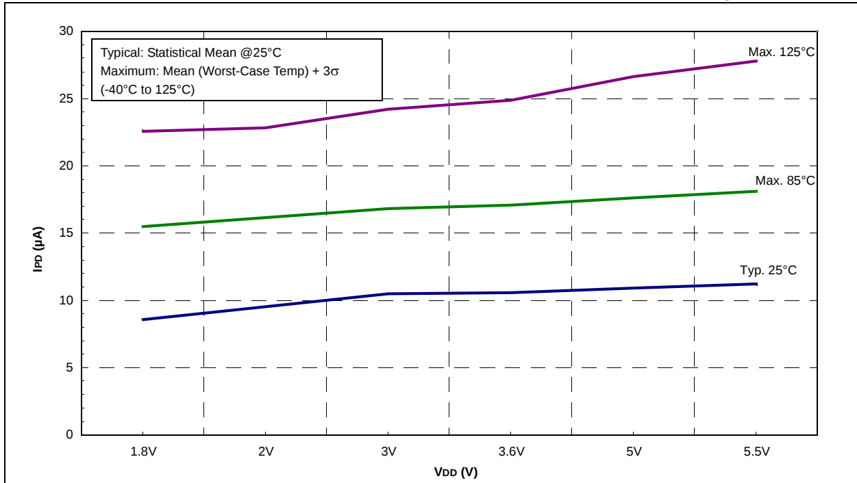
FIGURE 24-37: PIC16F72X CAP SENSE MEDIUM POWER I_{PD} vs. V_{DD} , V_{CAP} = 0.1\mu F
