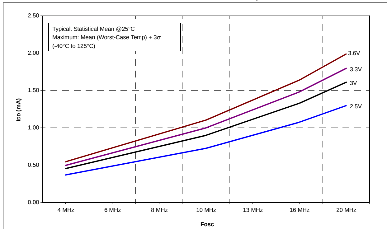
FIGURE 24-12: PIC16LF72X TYPICAL I_{DD} vs. F_{OSC} OVER V_{DD} , HS MODE
