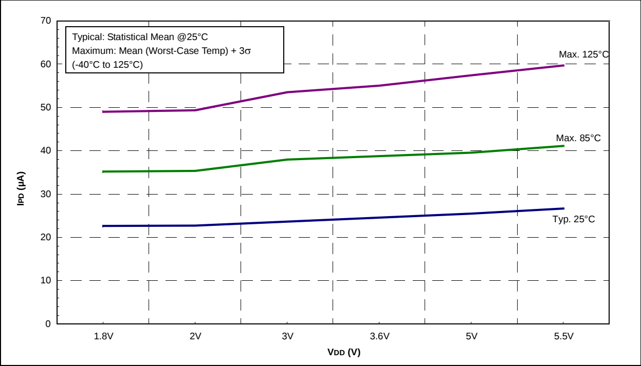
FIGURE 24-31: PIC16F72X FIXED VOLTAGE REFERENCE I_{PD} vs. V_{DD} , V_{CAP} = 0.1\mu F
