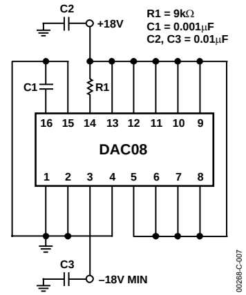
Figure 6. Burn-In Circuit
