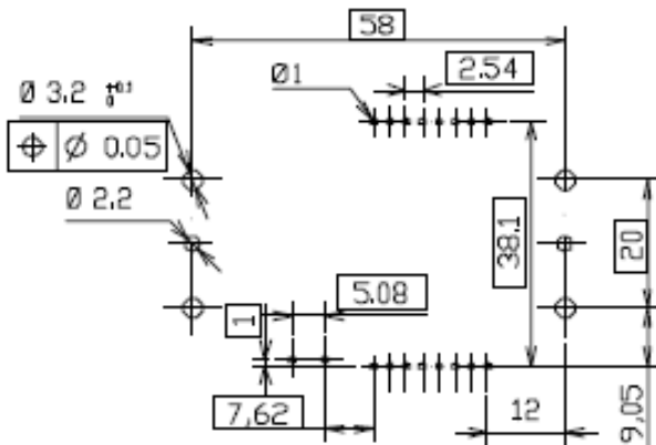
IMPLANTATION C.I PCB FOOTPRINT
