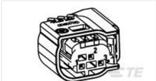
TE Part #1379729-1 3POS MQS REC SEALED COD A
