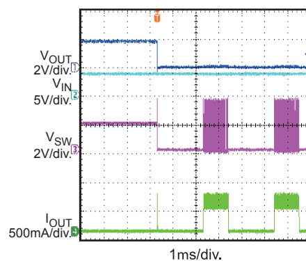
Short-Circuit Entry
