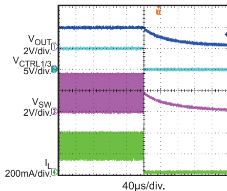
CTRL Off
