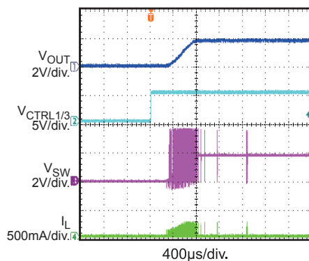
CTRL On
