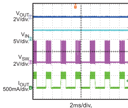
Short-Circuit Steady
