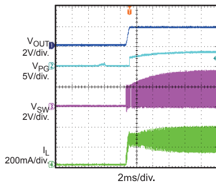
PG On
