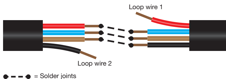
Soldering of a single multi-conductor cable
