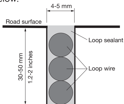
Loop with multiple turns
