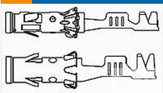
TE Part #1-929990-0 1,5MM SOCK CONTACT SWS
