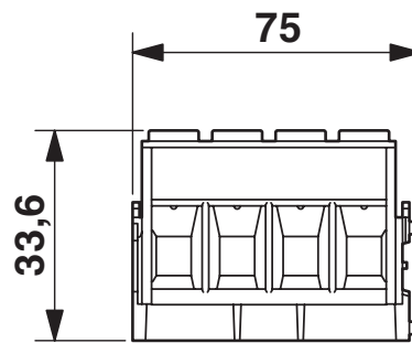
Dimensional drawing
